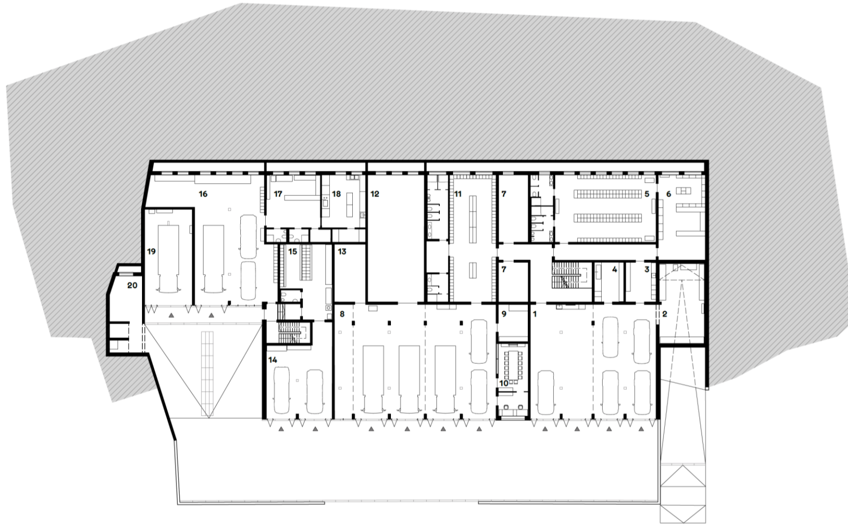
Erdgeschoss Piano terra
